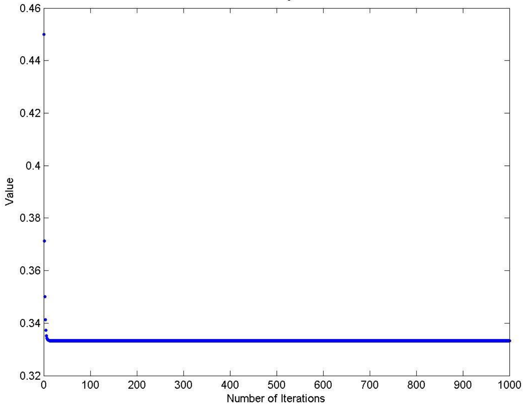
Logistic Equation, x_0=0.45 , \lambda=1.50
