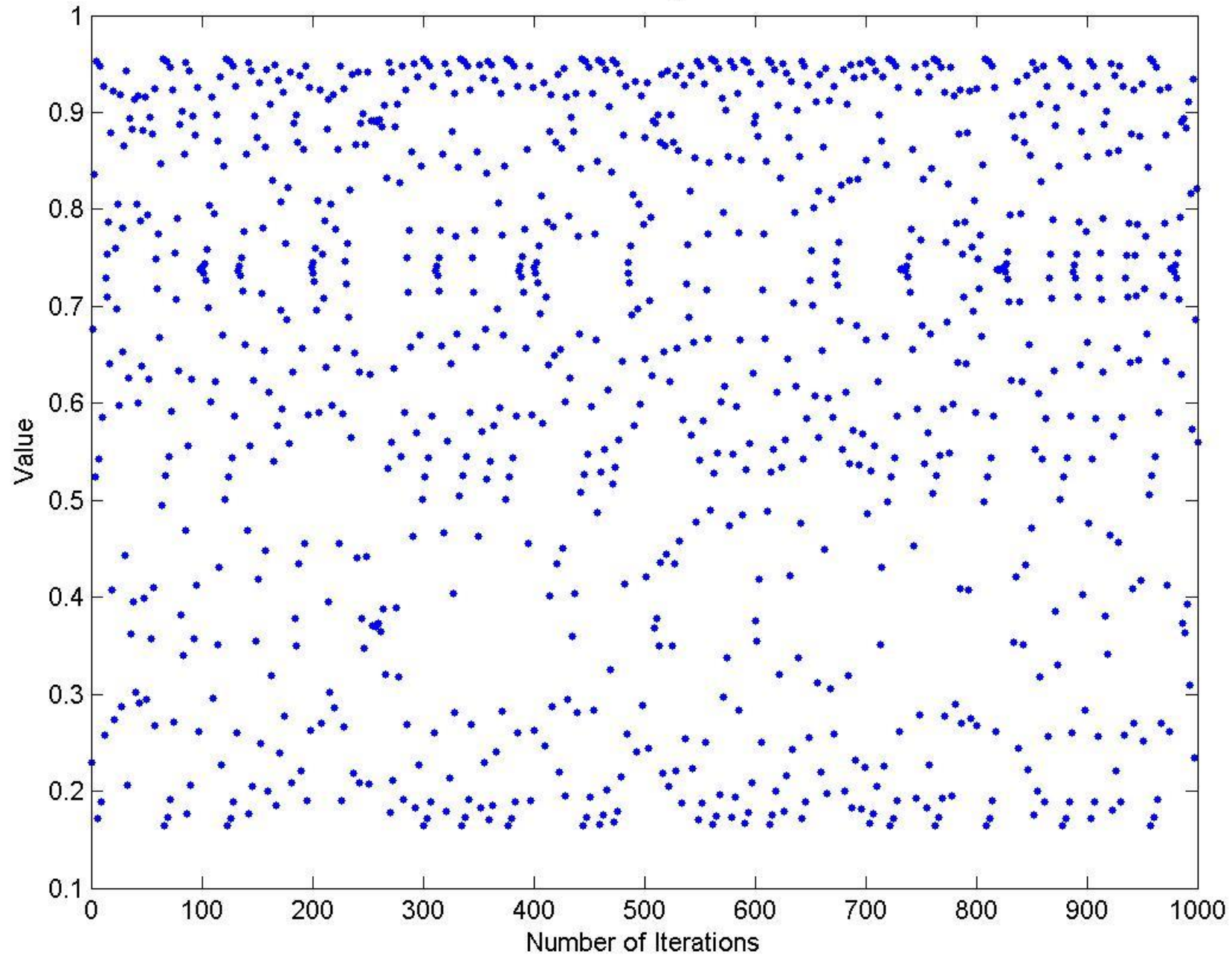
Logistic Equation, x_0=0.23 , \lambda=3.82
