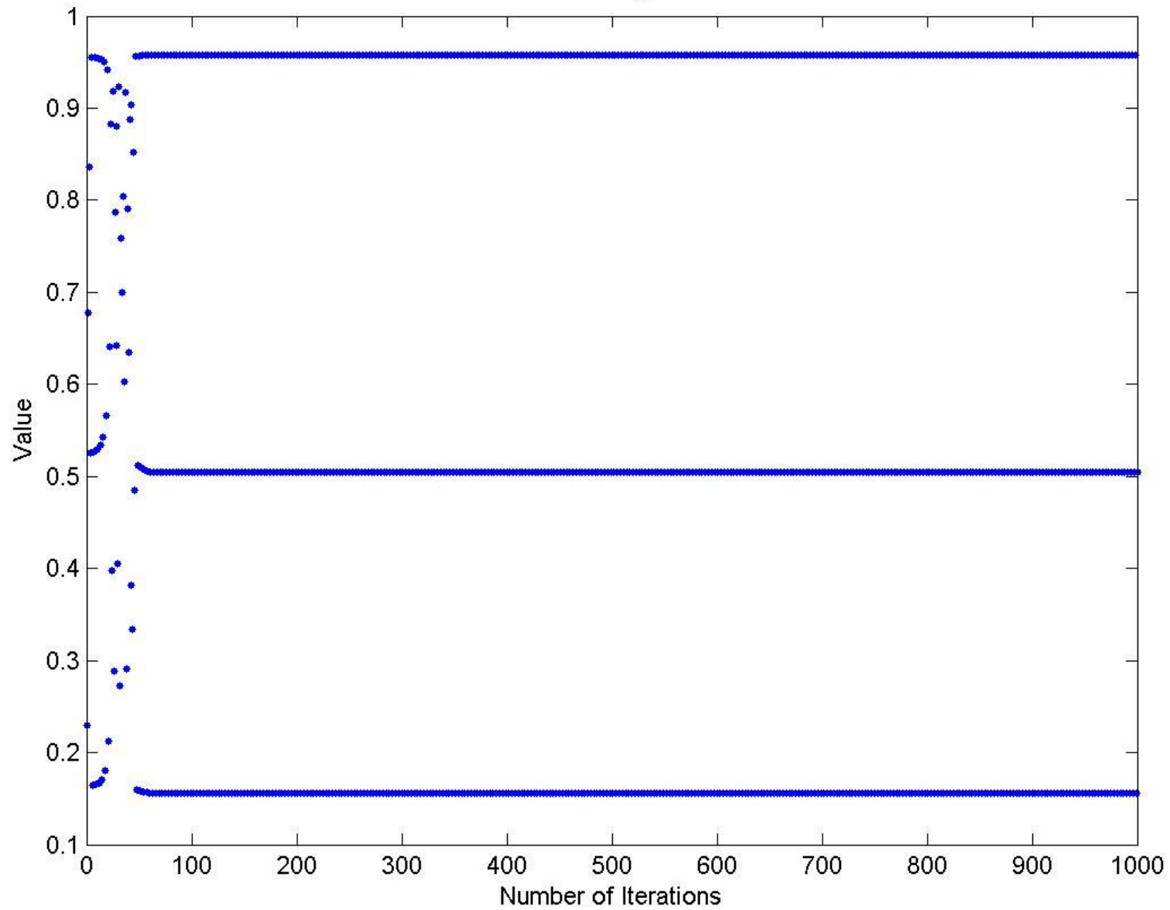
Logistic Equation, x_0=0.23 , \lambda=3.83
